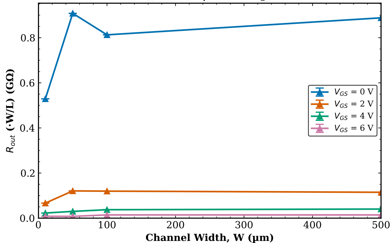
TFT1 Transistor 1 R_{out} vs W | L = 40\text{ }\mu\text{m}
